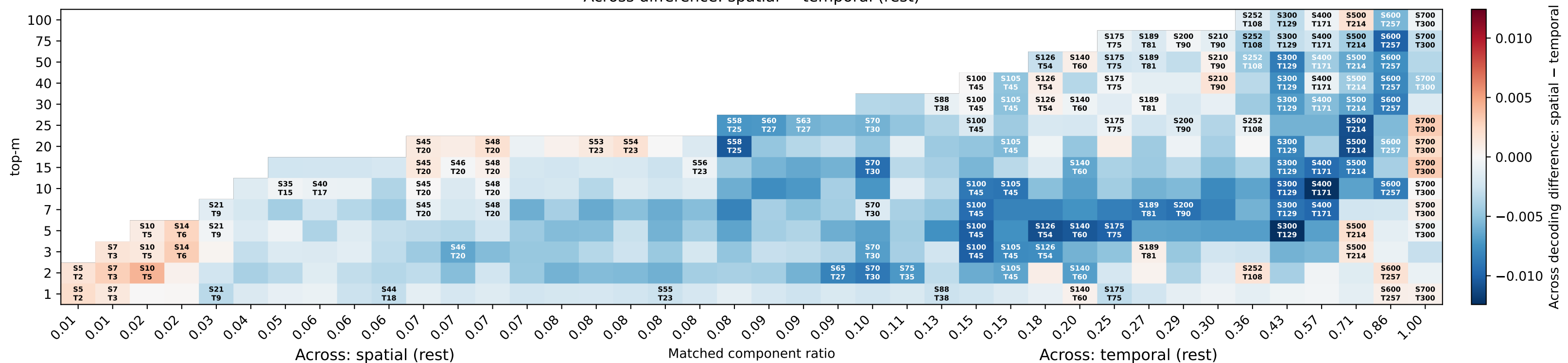
Across difference: spatial – temporal (rest)
