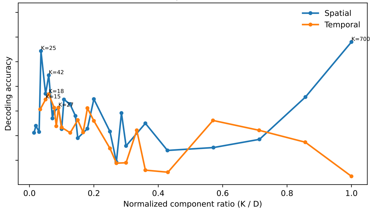
Within decoding (word) Top-m = 10
