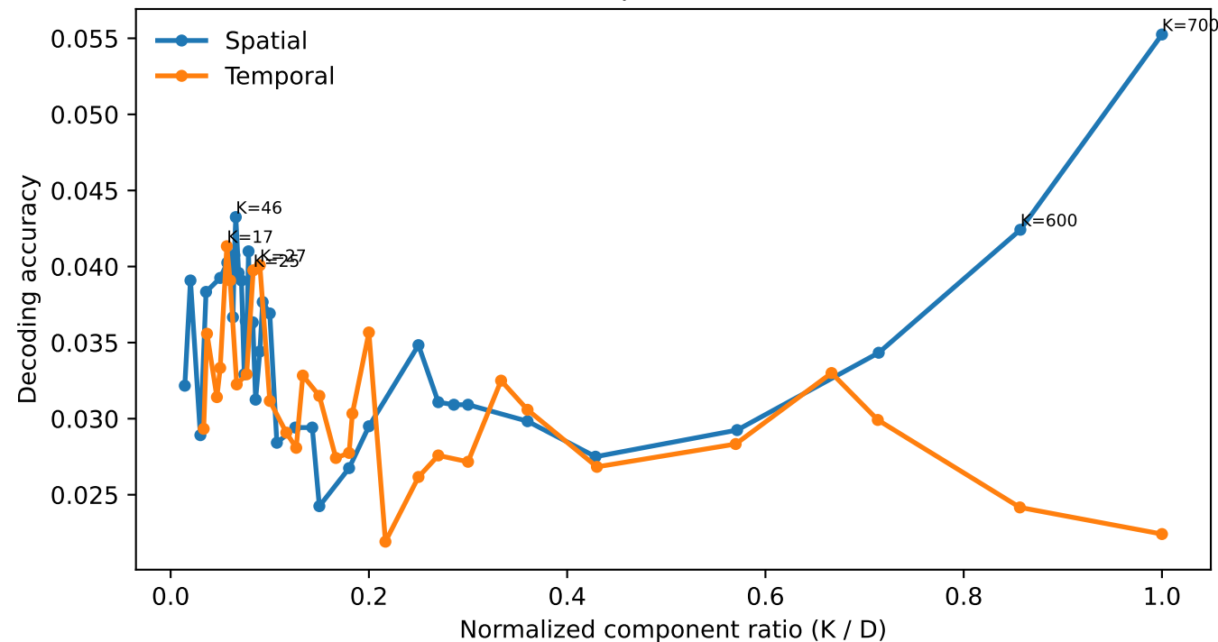
Across decoding (word) Top-m = 10
