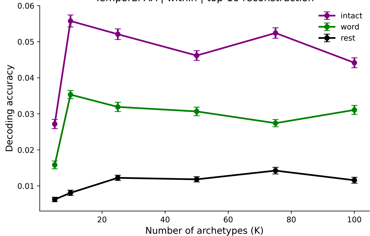
Temporal AA | within | top-10 reconstruction
