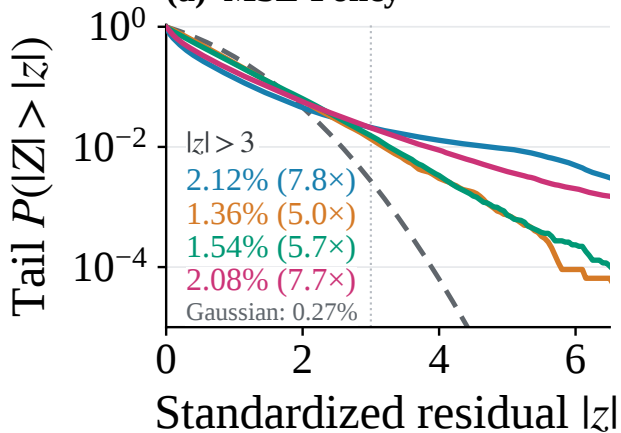
(a) MSE-Policy
