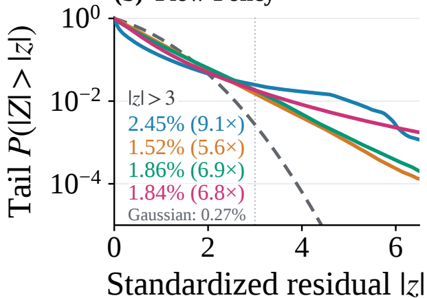
(b) Flow-Policy
