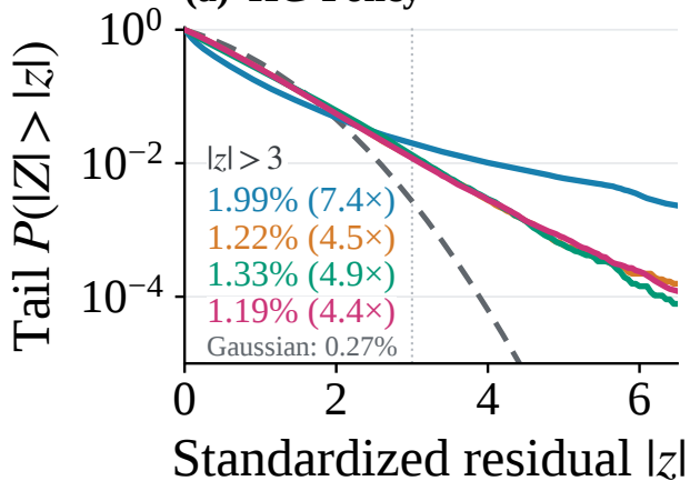
(a) HG-Policy
