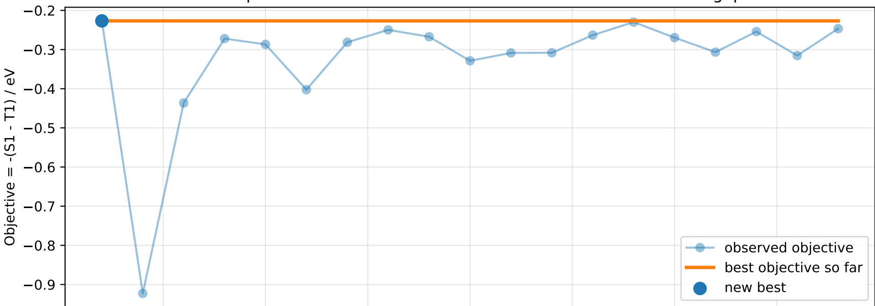
BO improvement curve: Pollice 2021 lowest-conformer TD-DFT gap
