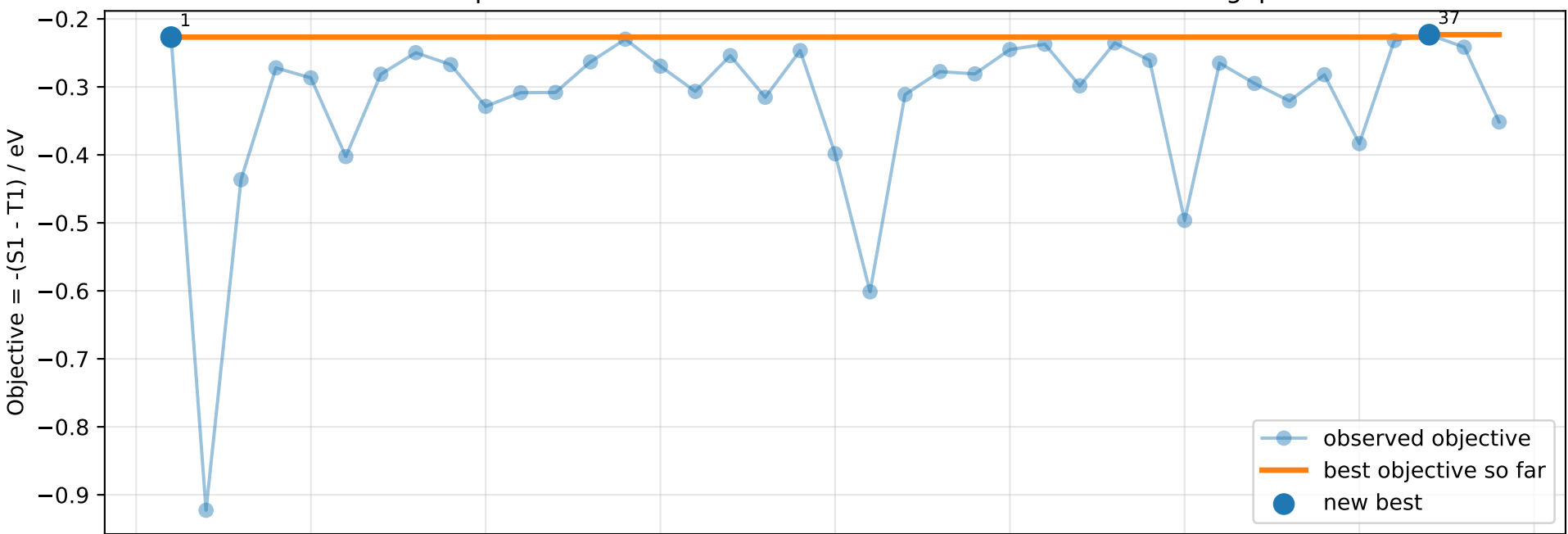
BO improvement curve: Pollice 2021 lowest-conformer TD-DFT gap
