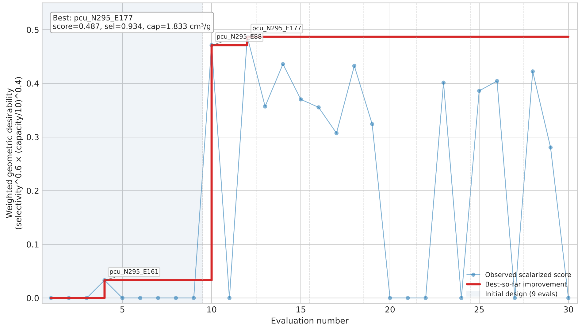
BO Improvement Curve: Xe/Kr PORMAKE MOF Campaign
