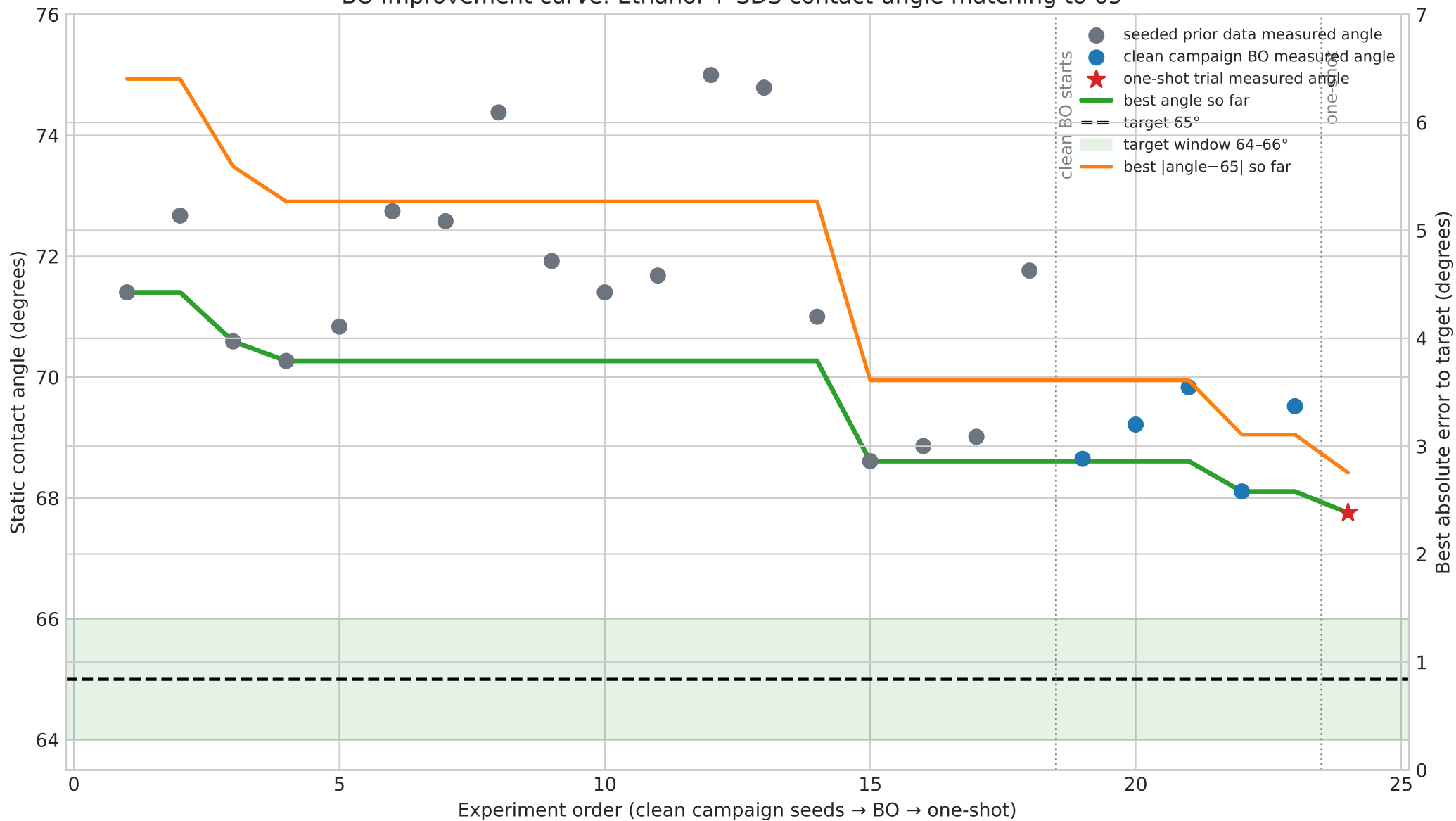
BO improvement curve: Ethanol + SDS contact-angle matching to 65°
