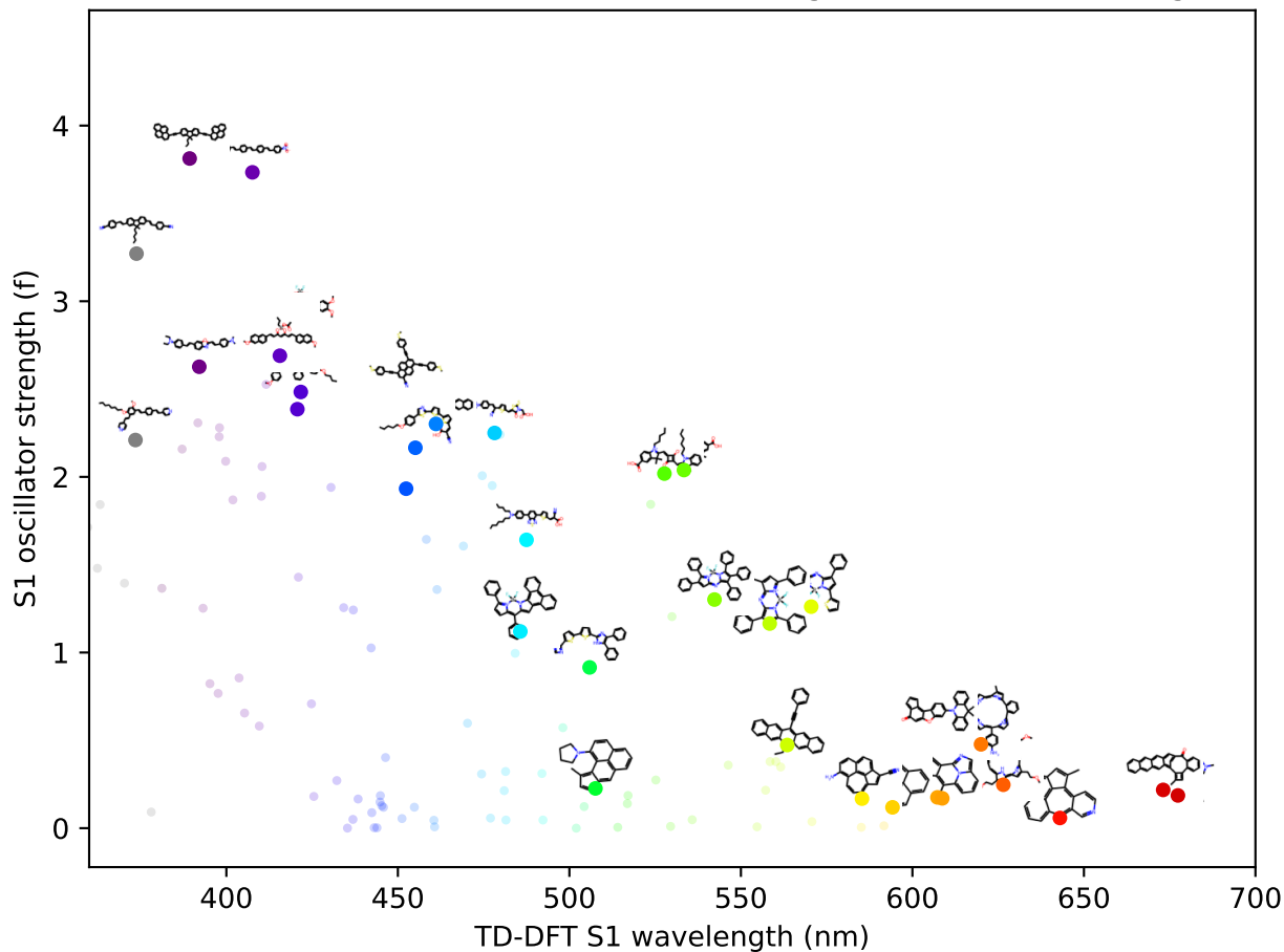
TD-DFT(SOC): Downselected S1 wavelength vs oscillator strength
