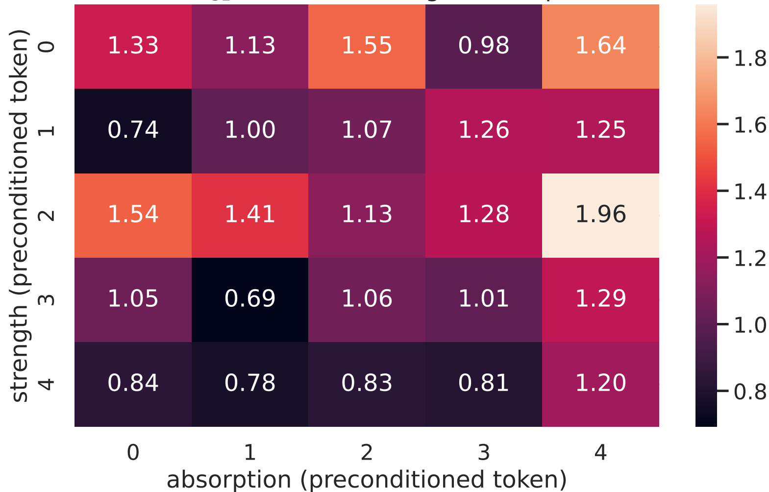
Std of E_{S1} (eV) over (strength, absorption)
