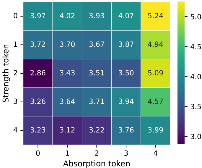
Median \Delta E_{S_0 \rightarrow S_1} (eV)
