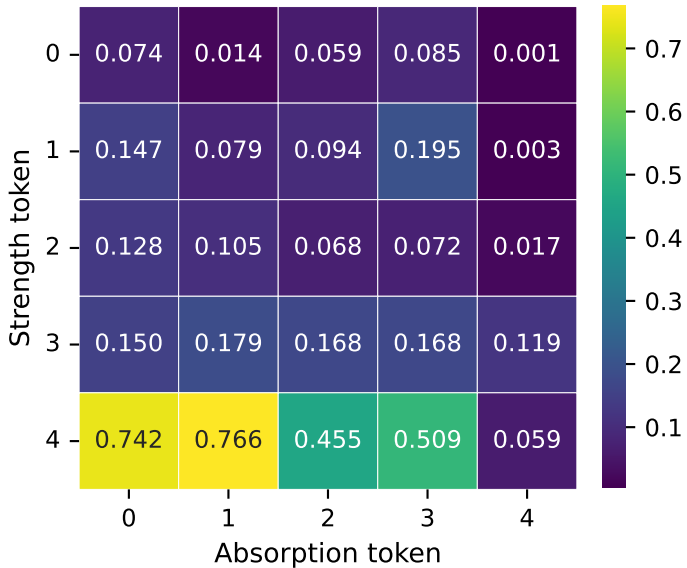
Median f_{S_0 \rightarrow S_1}
