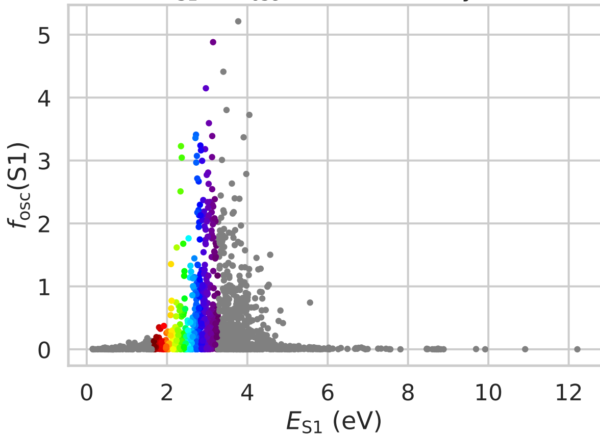
E_{S1} vs f_{osc}(S1) (colored by \lambda )
