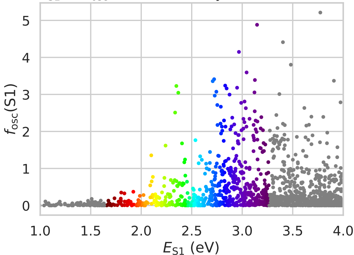
E_{S1} vs f_{osc}(S1) (colored by \lambda , zoom 1–4 eV)
