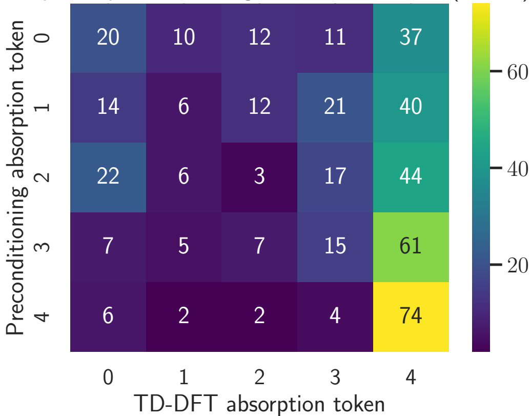
Absorption: preconditioning vs TD-DFT tokens (counts)
