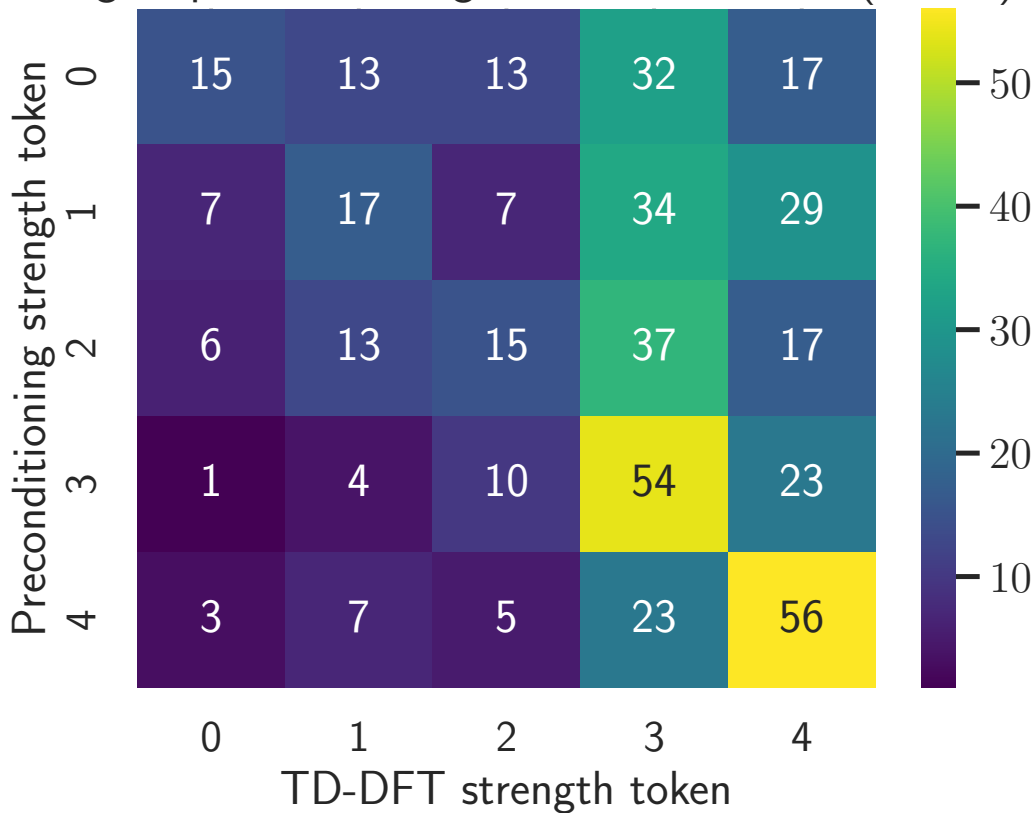
Strength: preconditioning vs TD-DFT tokens (counts)
