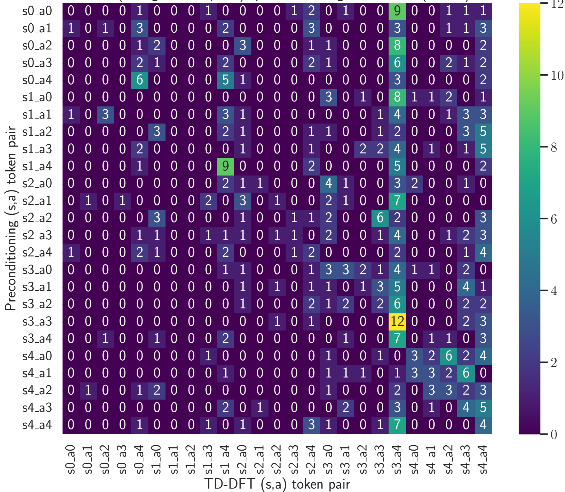
Joint (strength, absorption): preconditioning vs TD-DFT (counts)
