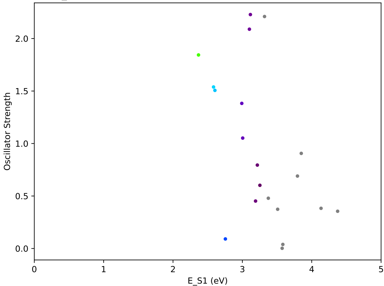
TD-DFT E_S1 vs Oscillator Strength (Strength Token=4, Absorption Token=0)
