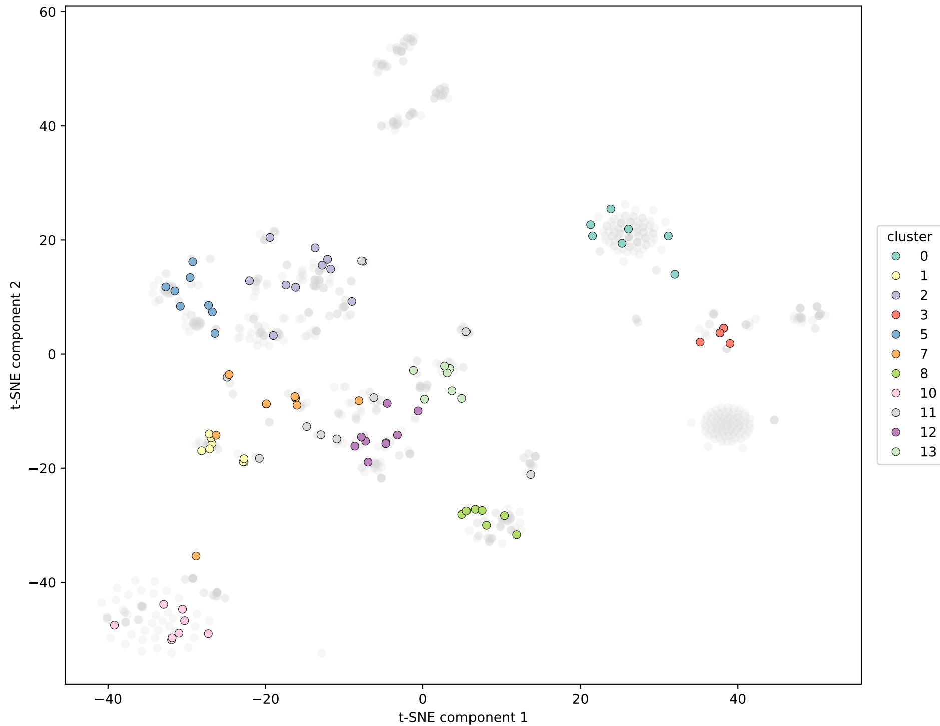
t-SNE of selected molecules
