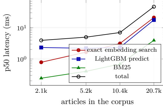
Figure 2: Per-stage median latency against corpus size, both axes logarithmic. The figures behind it are in Appendix D.
