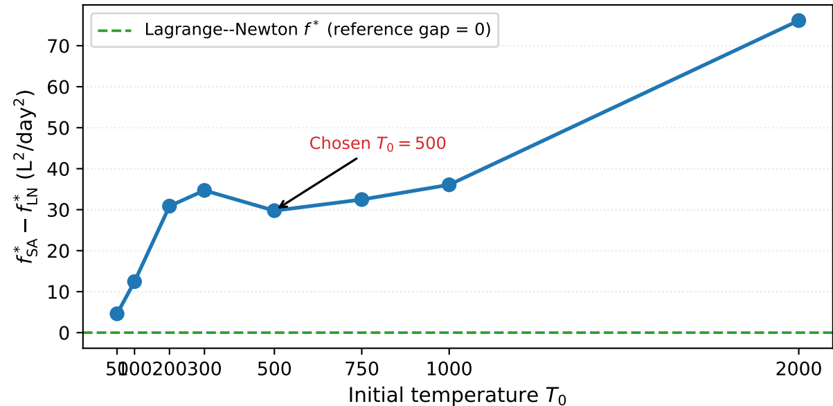
SA sensitivity to initial temperature T_0 ( k_{\max} = 50,000 , seed=42)
