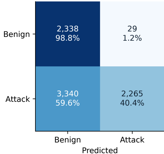
Frozen MLP
