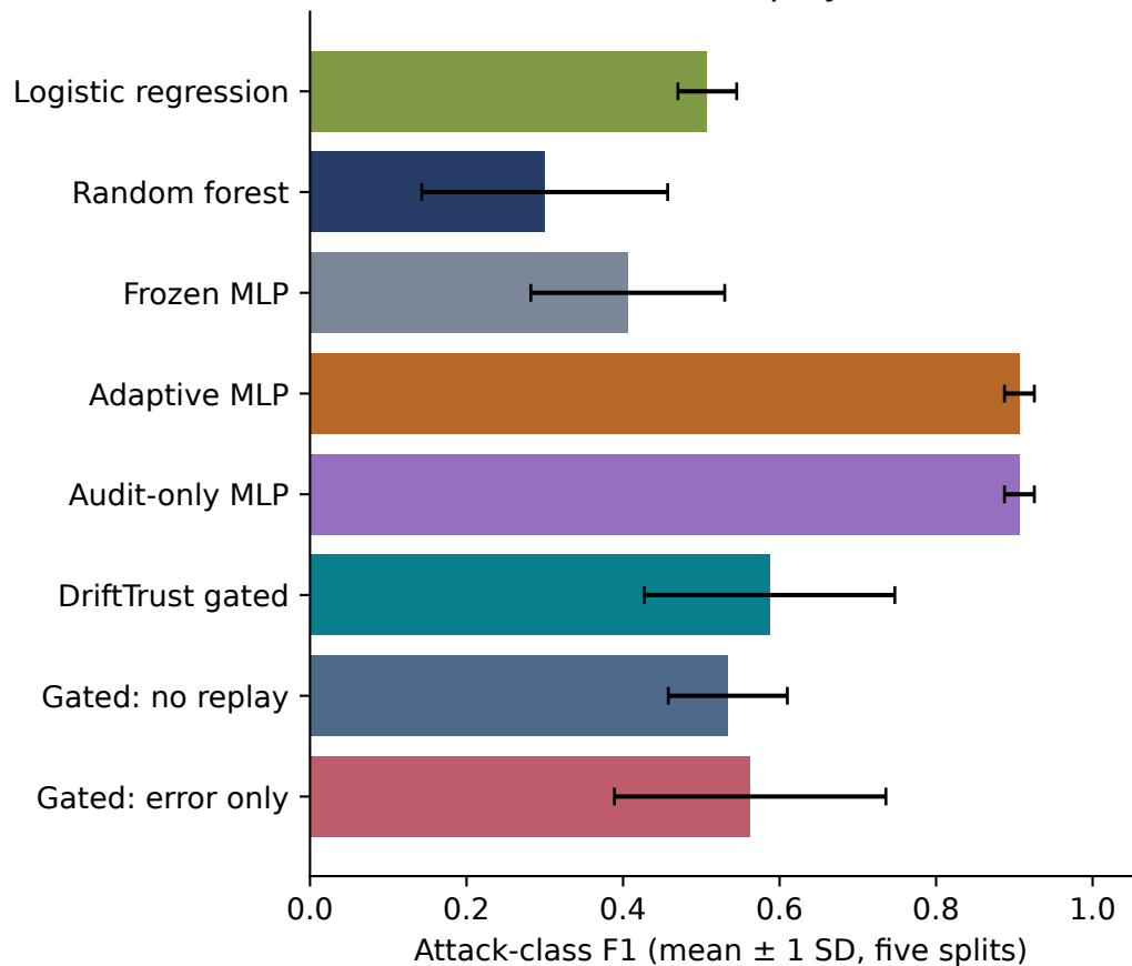
Shifted replay
