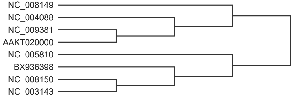
AFproject reference tree (yersinia_hgt)
