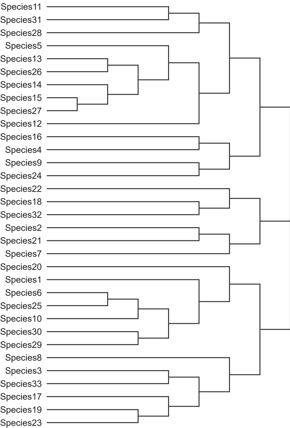
AFproject reference tree (sim_hgt)
