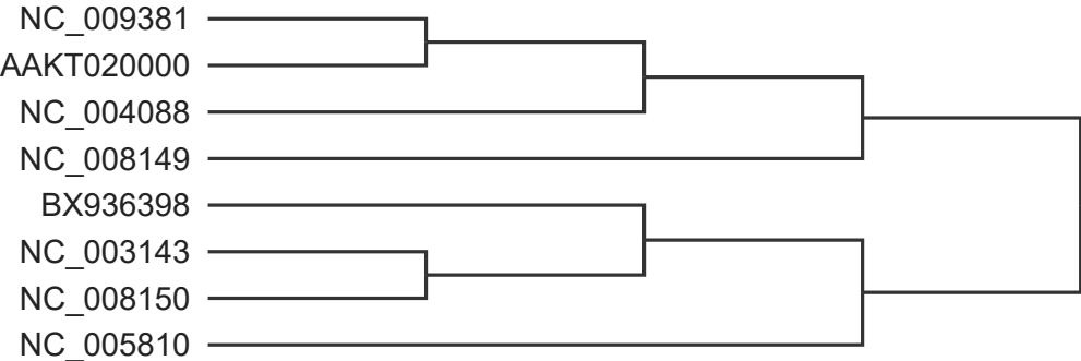
AFproject reference tree (yersinia_hgt)
