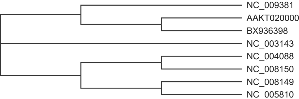
Q-MAWS tree
