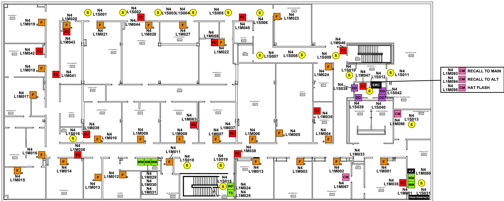
BASEMENT LEVEL 1
