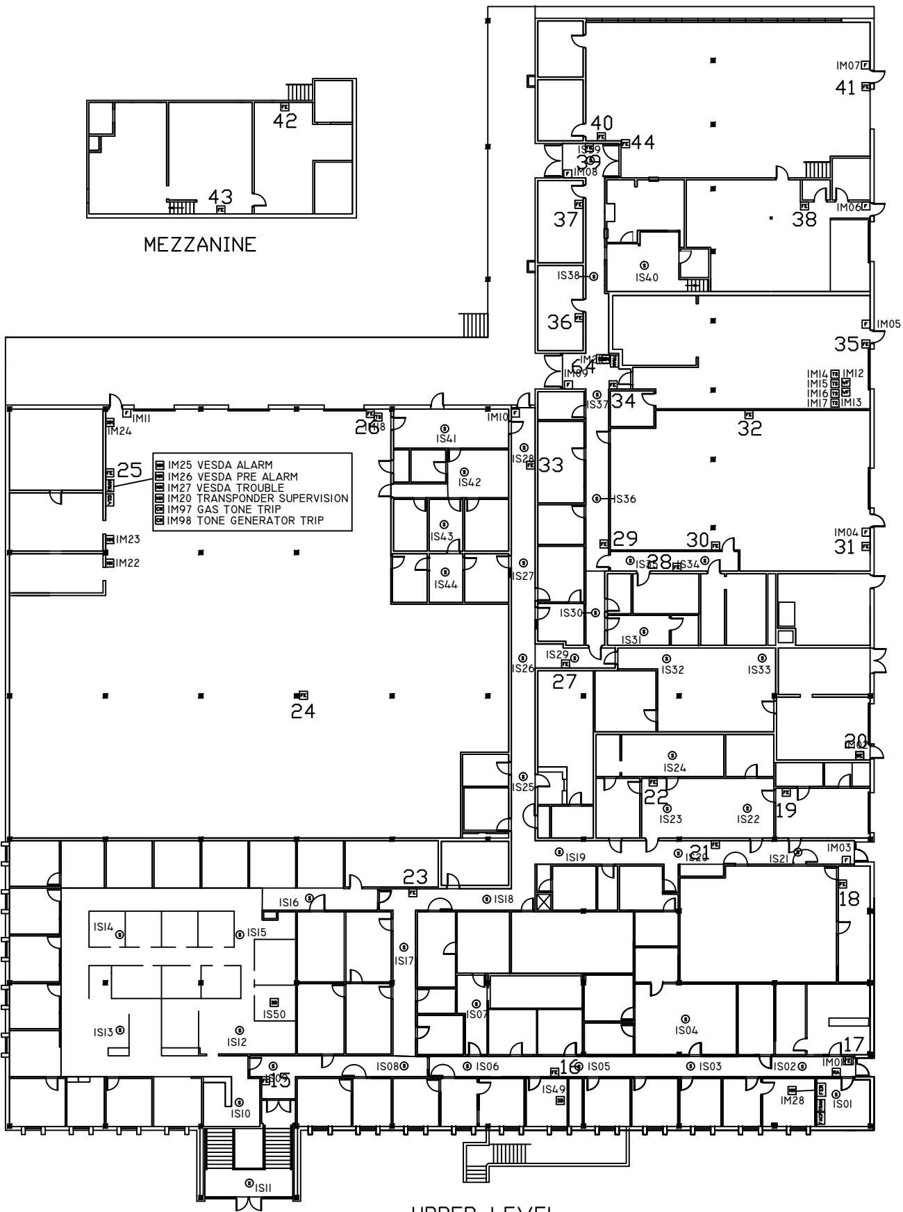
UPPER LEVEL
