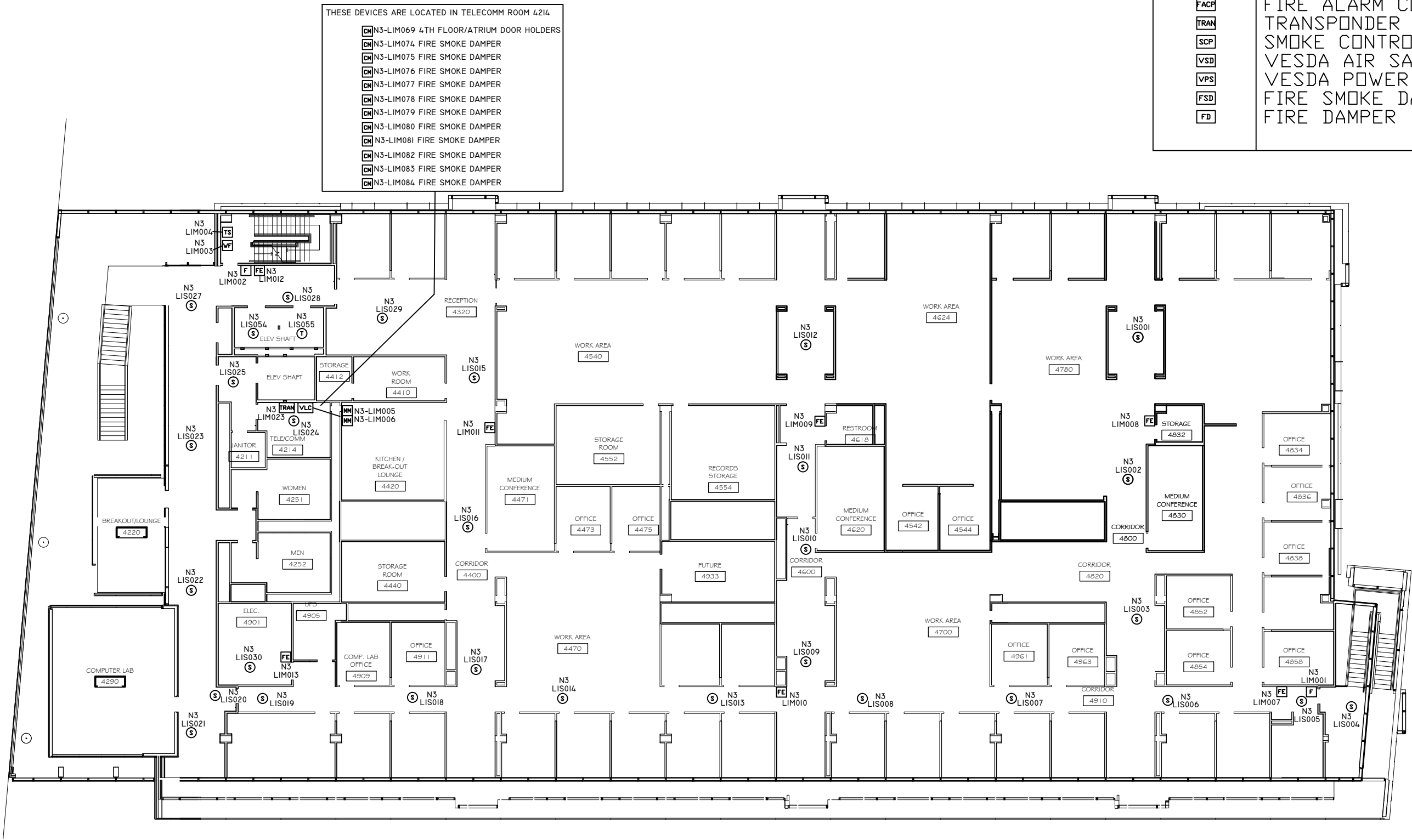
FOURTH FLOOR
