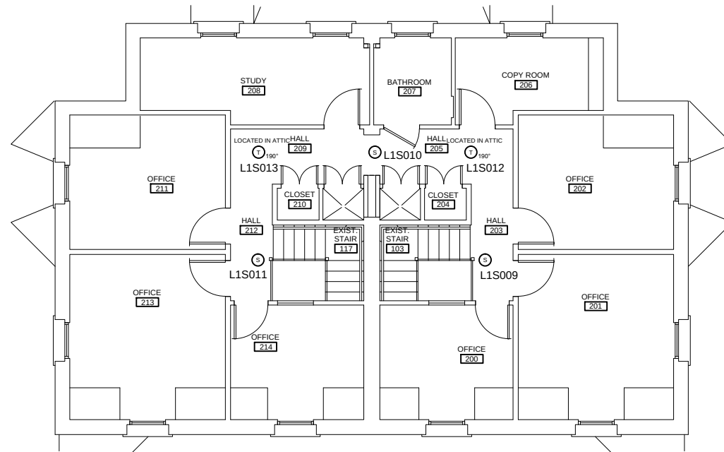
UPPER FLOOR
