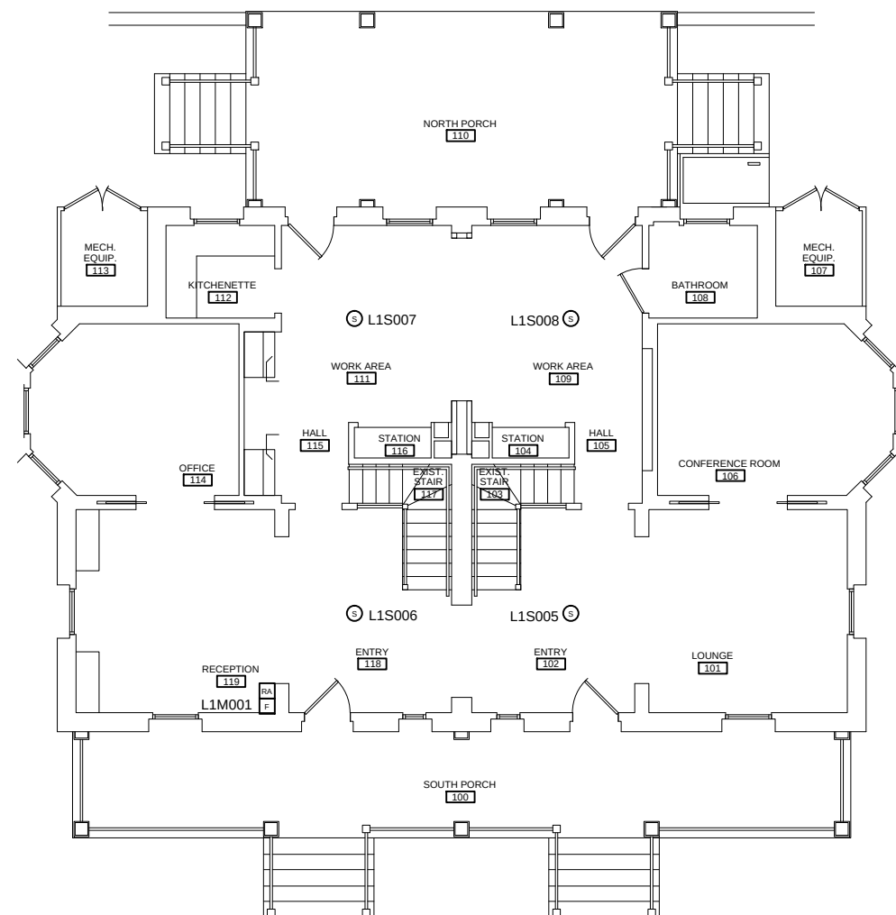
MAIN FLOOR
