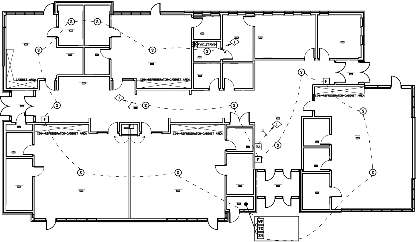
U OF U WEST VILLAGE HOUSING P2 - DAYCARE
