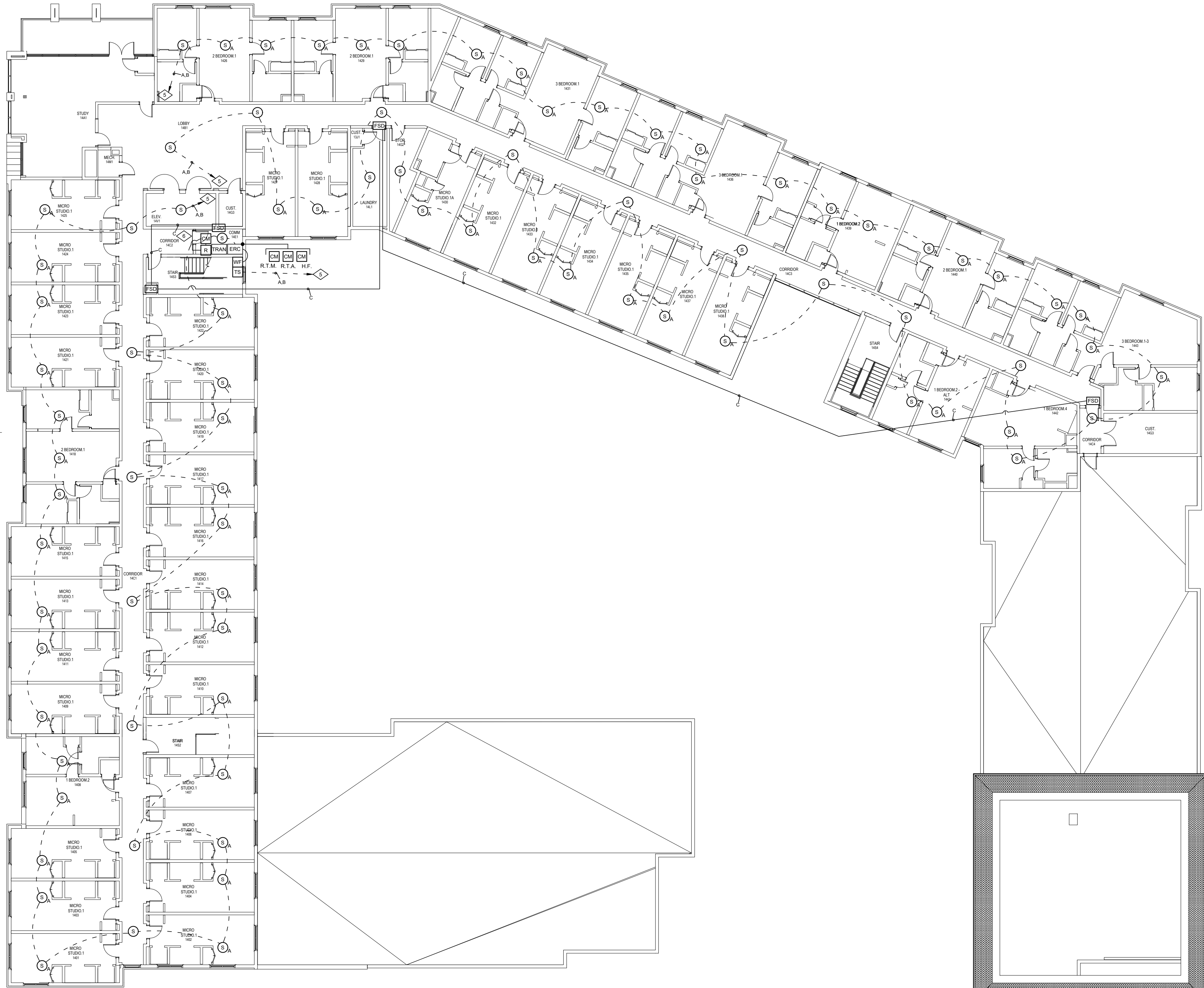
U of U WEST VILLAGE HOUSING - BLDG 'C' FOURTH FLOOR
