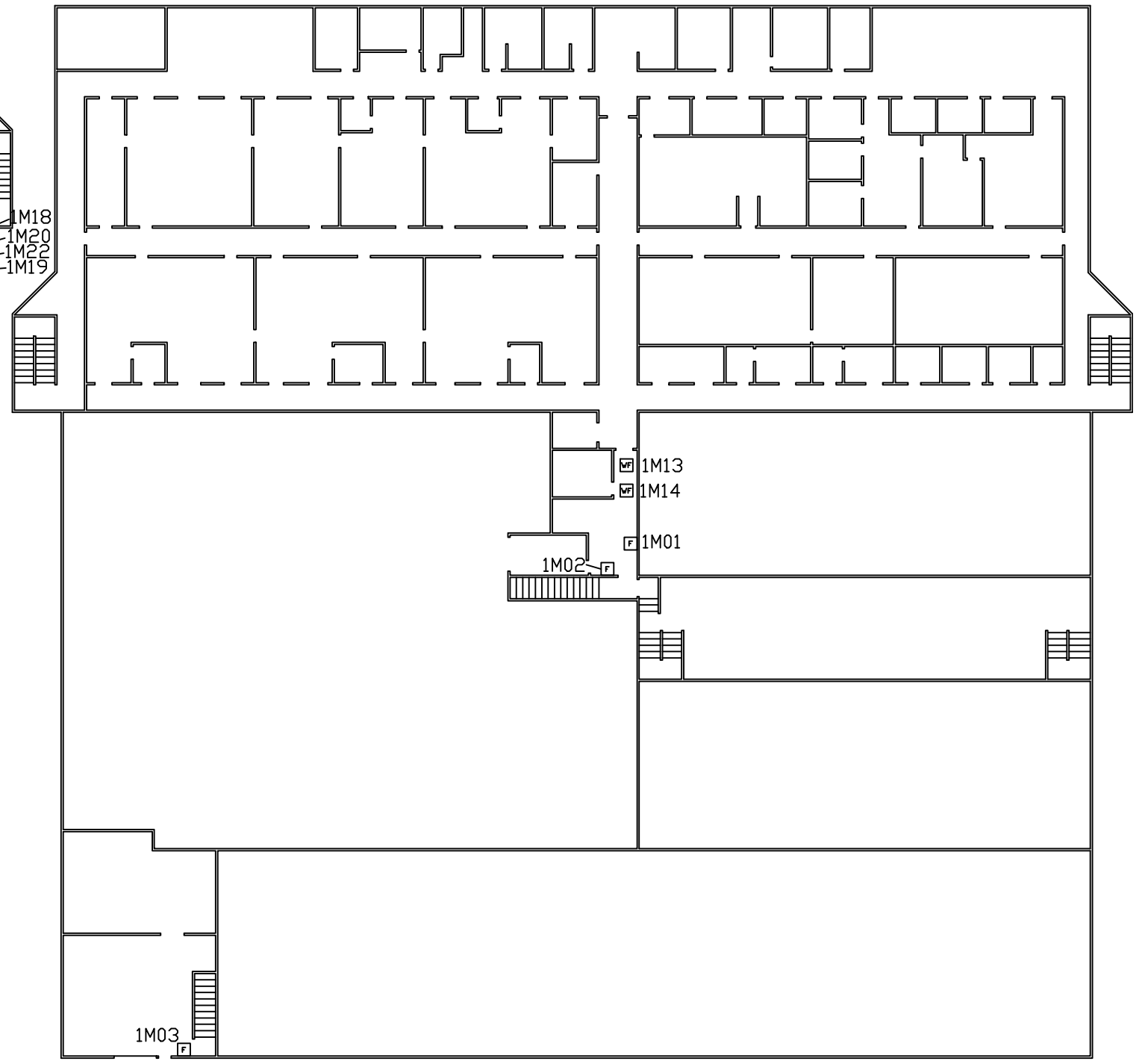
MEZZANINE LEVEL
