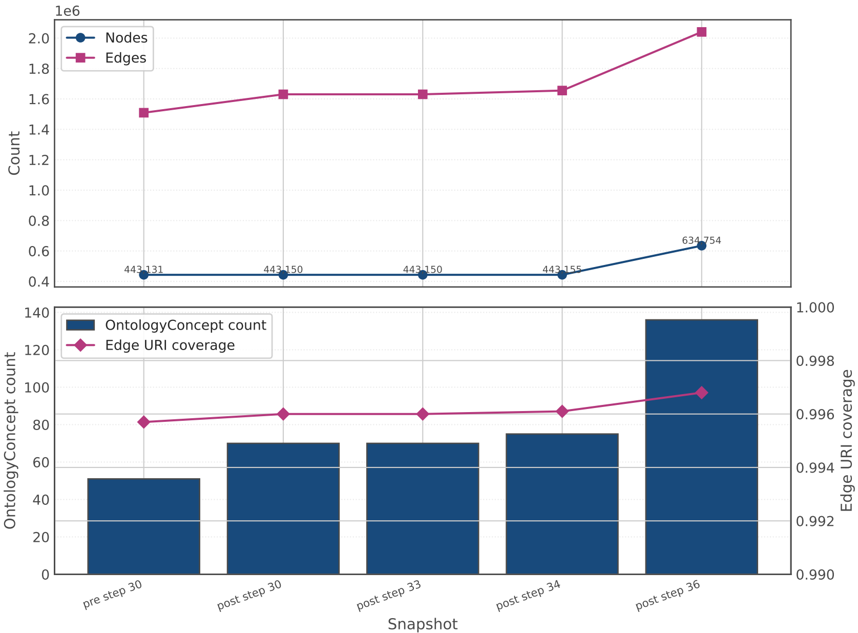
Cumulative deltas across enrichment passes
