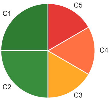
Query Distribution
