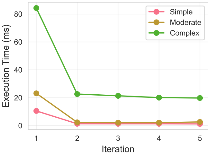
Performance Stability
