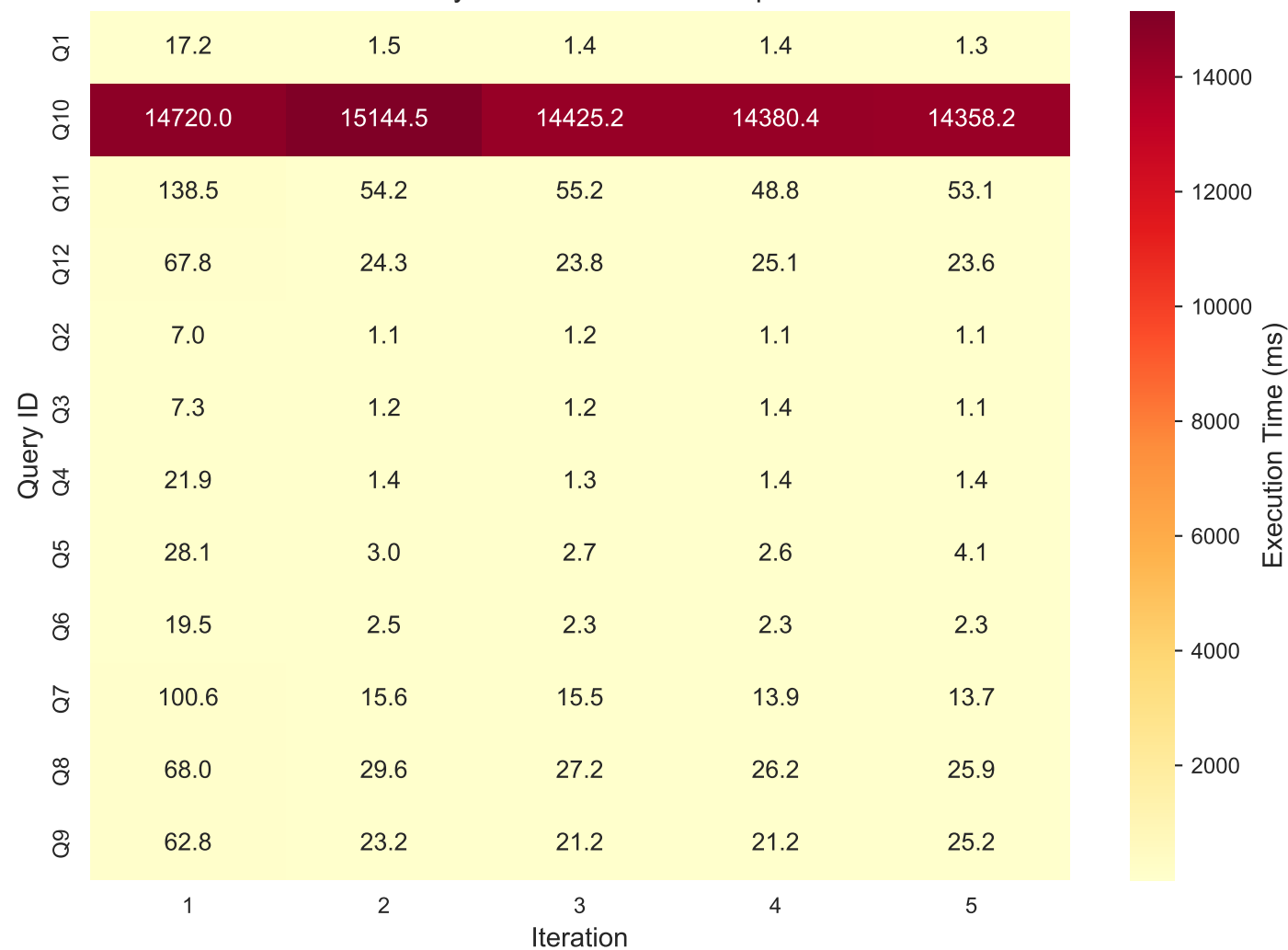
Query Distribution
