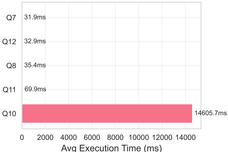
Top 5 Slowest Queries
