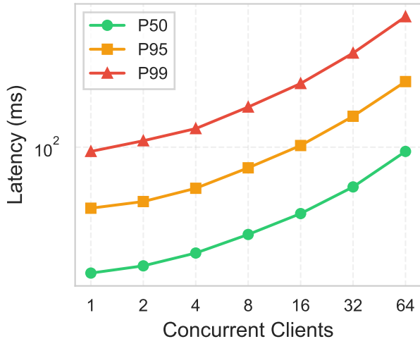
(b) Latency Percentiles
