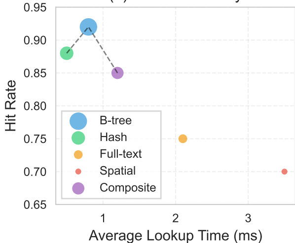
(a) Index Efficiency
