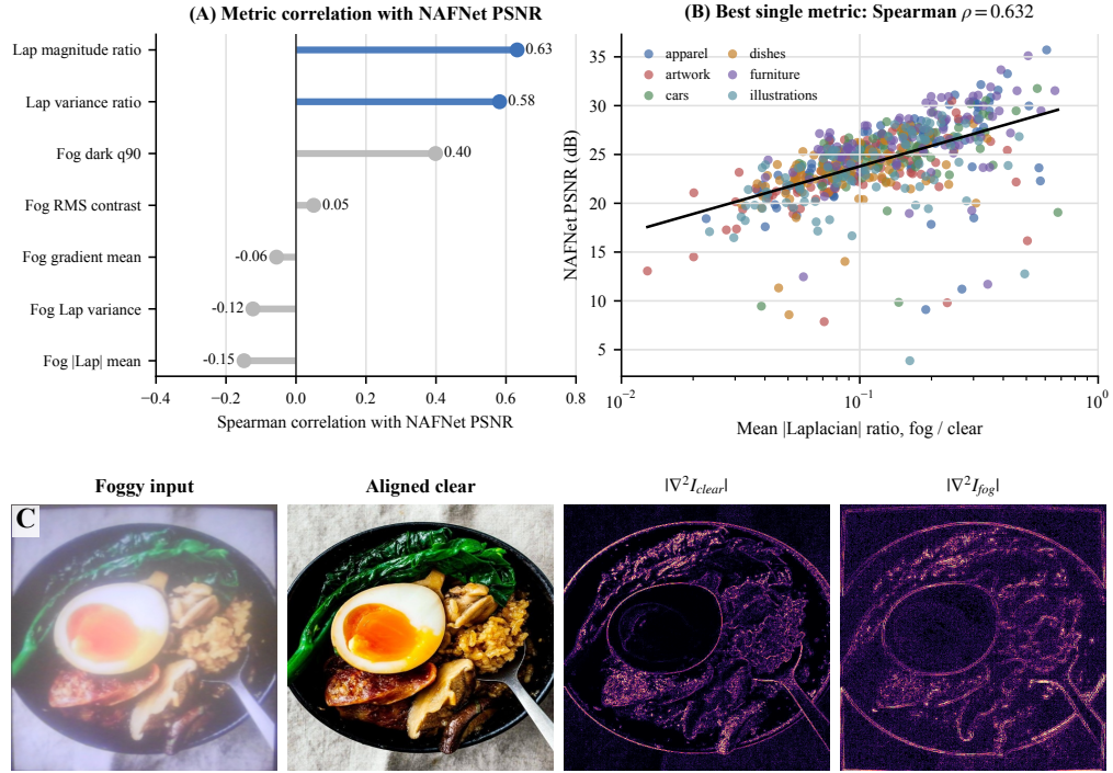
Fig. S6. Paired structure-loss metrics track NAFNet restoration difficulty on the fog-chamber held-out split. (A) Signed Spearman correlations between selected paired and foggy-only image statistics and per-image NAFNet PSNR, with \rho values labeled next to each point. (B) Per-image NAFNet PSNR plotted against the strongest single metric, the scalar fog/clear mean absolute Laplacian-response ratio. Points are colored by archive category, and the black line shows a fit versus \log_{10} of the metric. (C) Example showing the foggy input, aligned clear target, and independently contrast-scaled absolute Laplacian-response maps for clear and foggy images.
