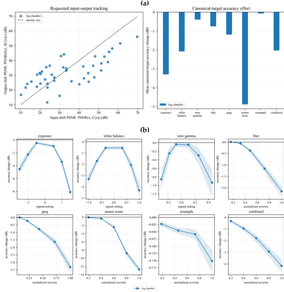
Fig. S7. Controlled synthetic-camera sensitivity of the fixed fog-chamber NAFNet check-point. (a) Left: condition-mean input-shift versus output-shift PSNR for the 42 nonidentity settings; the dashed line denotes equal input and output change, not a regression fit. Right: mean canonical-target accuracy change grouped by perturbation family. (b) Canonical-target accuracy change as a function of signed setting or normalized severity; shaded bands are 95% image-bootstrap confidence intervals.
