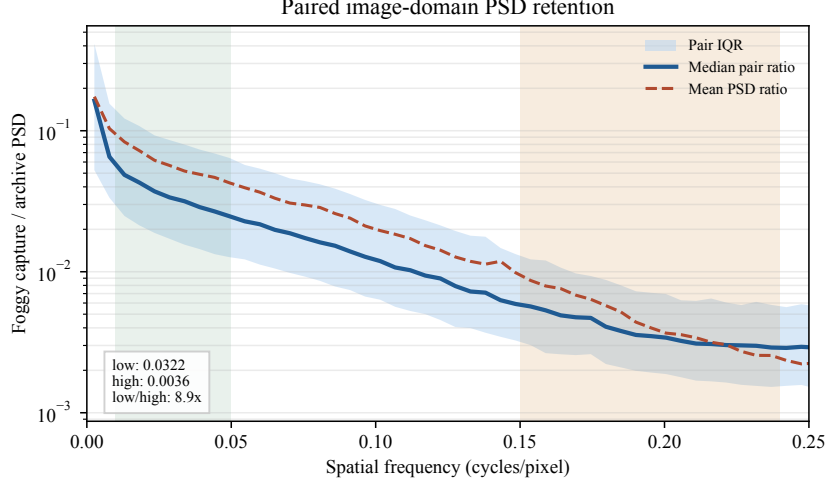
Fig. S5. Paired image-domain power-spectral-density retention for the held-out chamber split. The solid line shows the median foggy-capture/archive PSD ratio across image pairs; the shaded band shows the interquartile range. The dashed line shows the ratio of mean foggy and archive PSDs. Green and orange bands mark the low- and high-frequency ranges summarized in the text.
