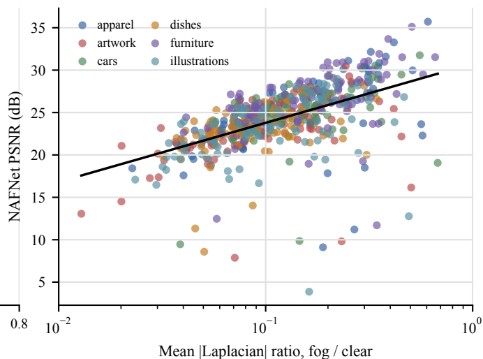
(B) Best single metric: Spearman \rho = 0.632
