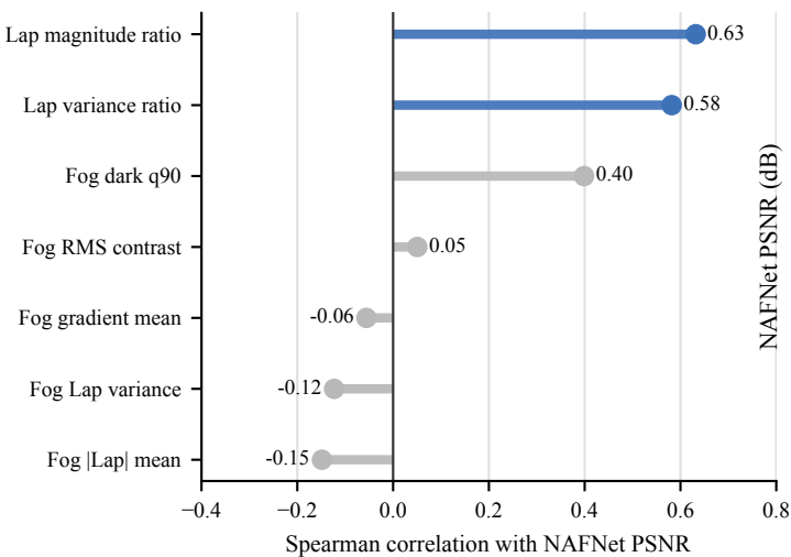
(A) Metric correlation with NAFNet PSNR
