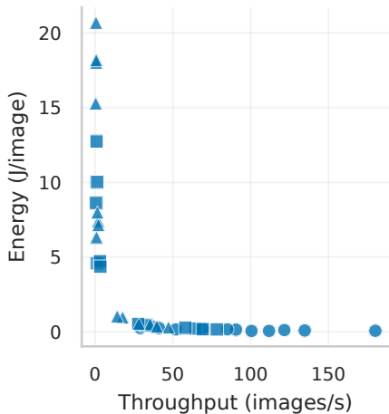
Apple M4 (Combined SoC)
