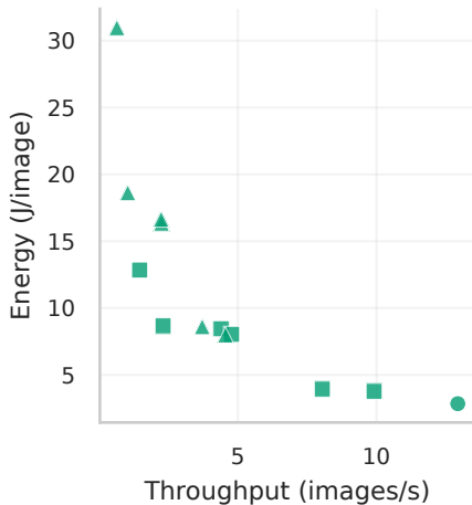
Intel i7-11800H (CPU package)
