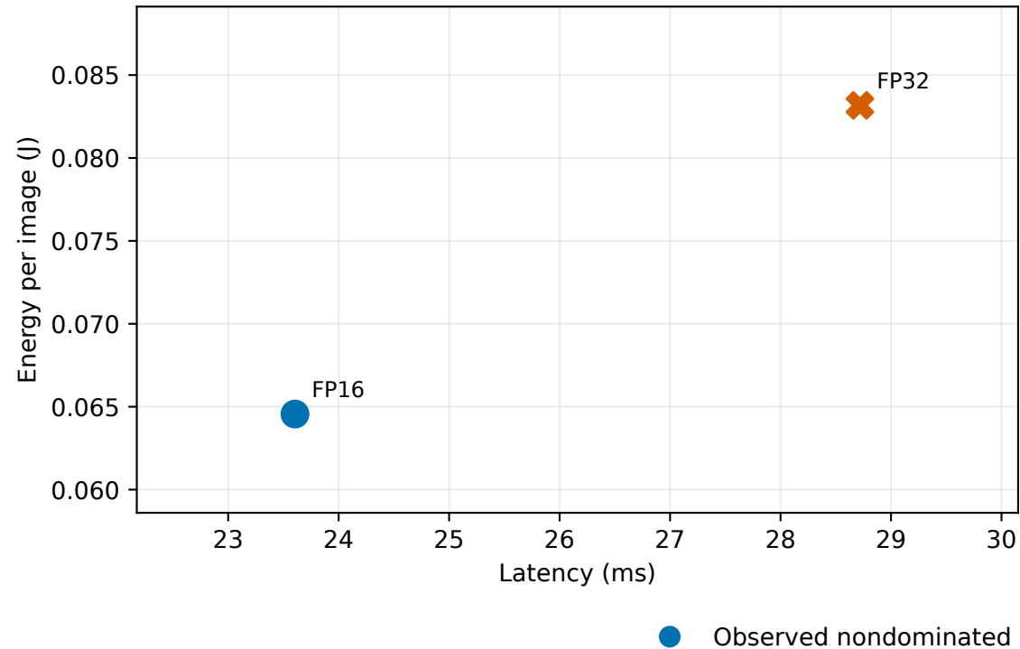
ResNet50 medium | Apple M4 / MPS Energy boundary: combined_soc
