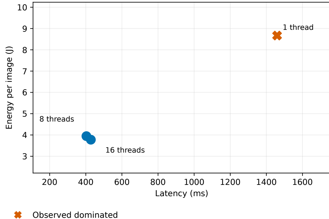
ConvNeXt-Base medium | Intel i7 CPU Energy boundary: cpu_package
