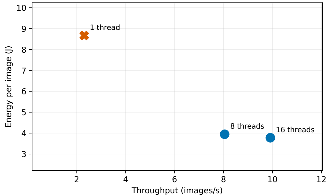
ConvNeXt-Base medium | Intel i7 CPU Energy boundary: cpu_package
