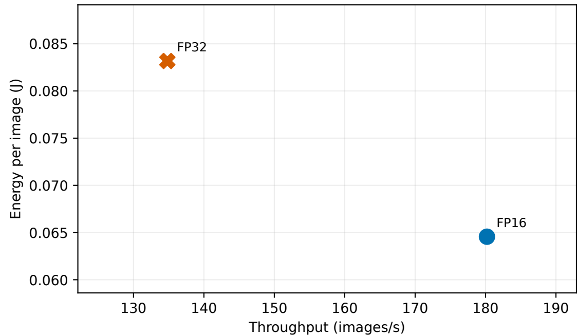
ResNet50 medium | Apple M4 / MPS Energy boundary: combined_soc
