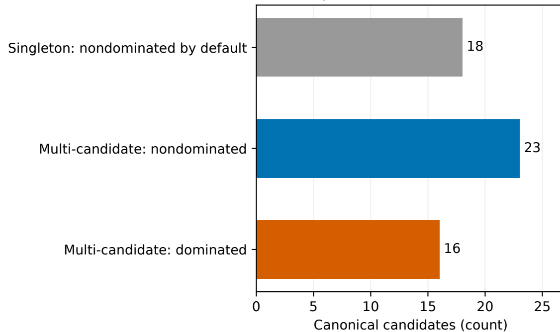
Group-local Pareto classification
