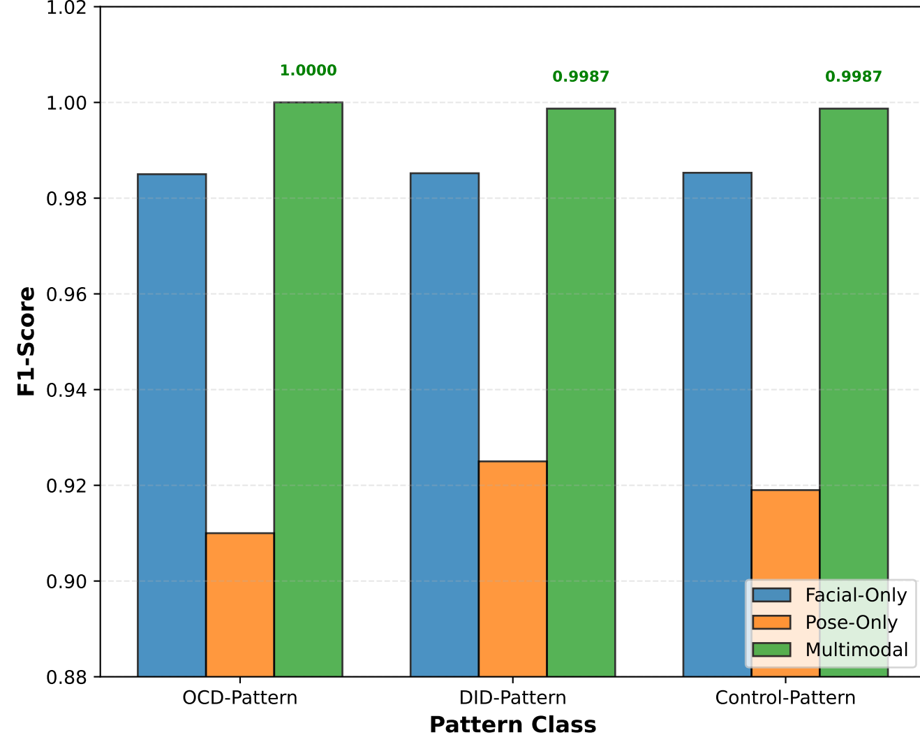
Per-Class F1-Scores Across Models
