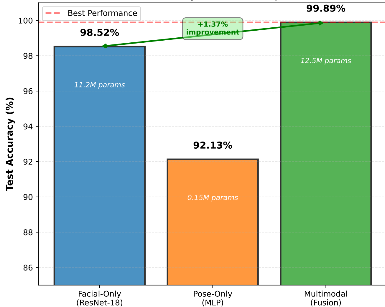
Ablation Study: Model Comparison
