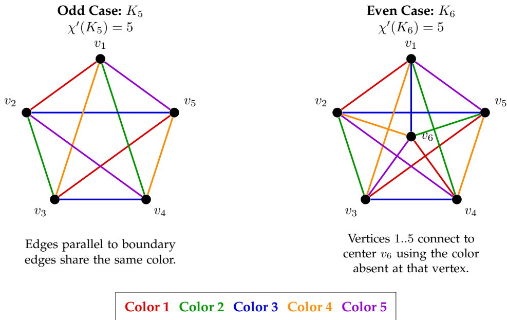
Figure 1.5: Coloring of K_5 and K_6
