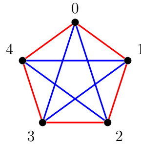
Decomposition of K_5
