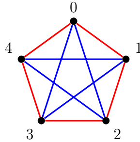
Decomposition of K_5
