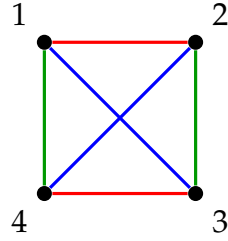
Decomposition of K_4
