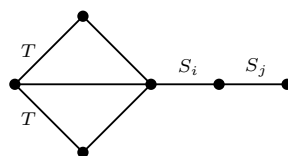
Figure 3.9: The clique configuration used in the proof of Theorem 3.1.10.
