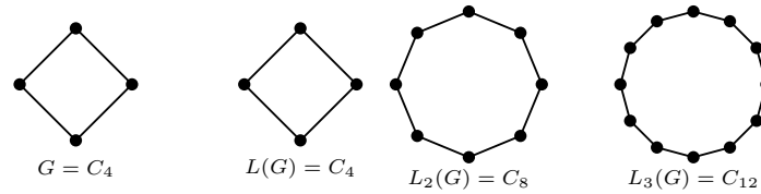
Figure 3.15: For a cycle, subdividing every edge increases its length; in particular, L_2(C_4) = C_8 but L^2(C_4) = C_4 .
