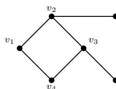
Figure 3.13: The cycle v_1 v_2 v_3 v_4 v_1 is a dominating closed trail.
