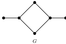
Figure 3.14: A non-Hamiltonian graph with a Hamiltonian edge graph.
