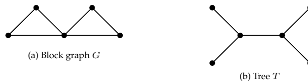
Figure 3.11: A block graph formed by two triangles sharing one vertex, and a tree T whose edge graph is isomorphic to it.
