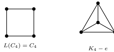
Figure 3.5: The edge graphs of the first two possibilities in Figure 3.4.
