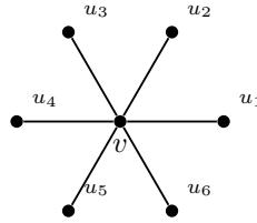
Figure 3.18: The neighbourhood of the central vertex of a star.
