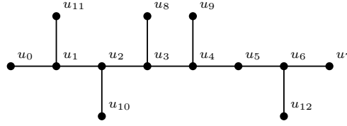
Figure 3.17: A tree realizing the eccentricity sequence [4^2, 5^4, 6^3, 7^4] .
