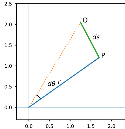
Differential arc-length element in polar coordinates
