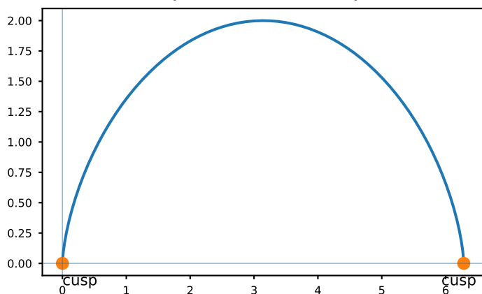
One arch of a cycloid: x = a(\theta - \sin \theta) , y = a(1 - \cos \theta)
