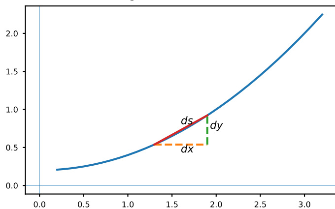
Differential arc-length element in Cartesian coordinates
