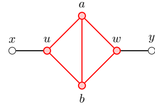
(All new vertices degree 3)
